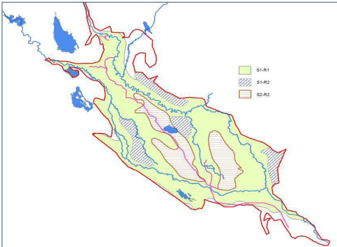
Figure (1) Mesopotamia Plain Soil Degradation Rate (FAO, 2011)
